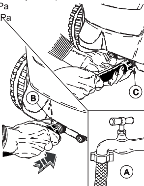
Raccordement hydraulique.
