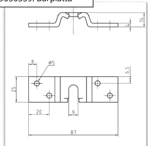
9056559: Bärplatta
