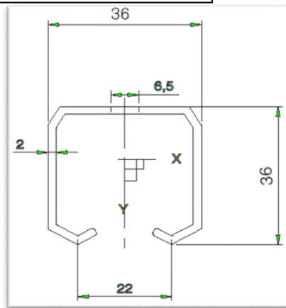
9056688: Portskena
