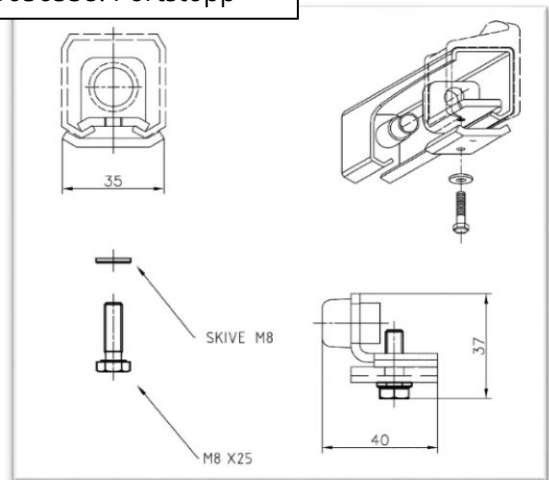
9056558: Portstopp
