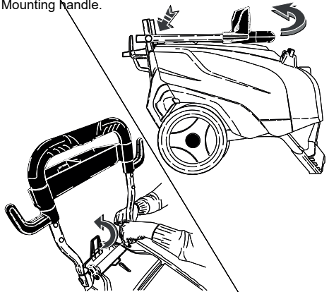
Mounting handle.
