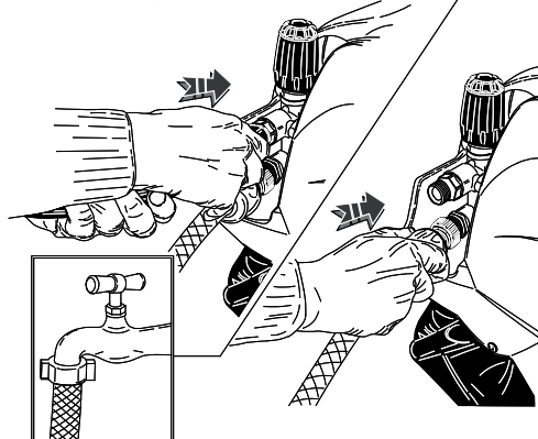
Raccordement hydraulique.
