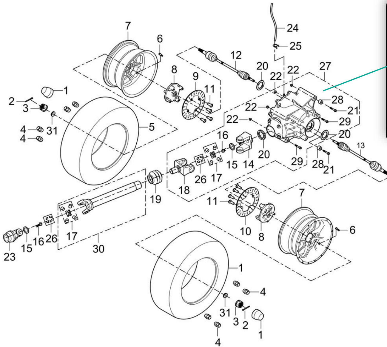
FIGUR 2 – Bakre differential (bakre drivsystem)
