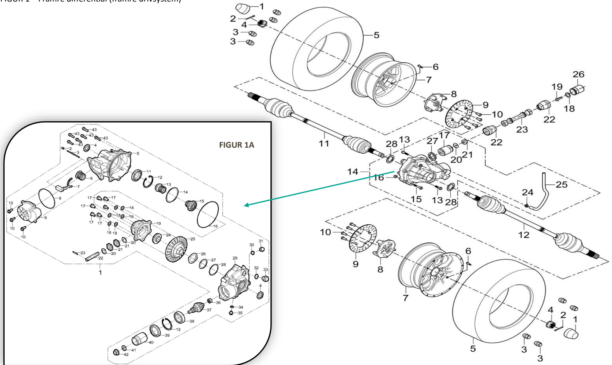
FIGUR 1 – Främre differential (främre drivsystem)
