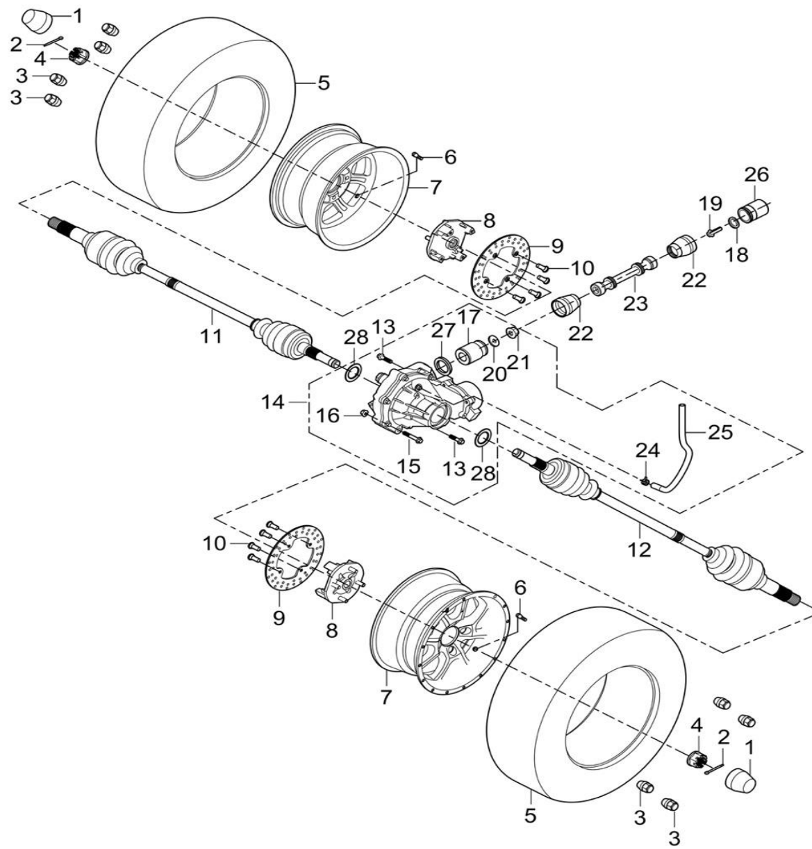
Fig 1: Drivenhet/Främre drivsystem
