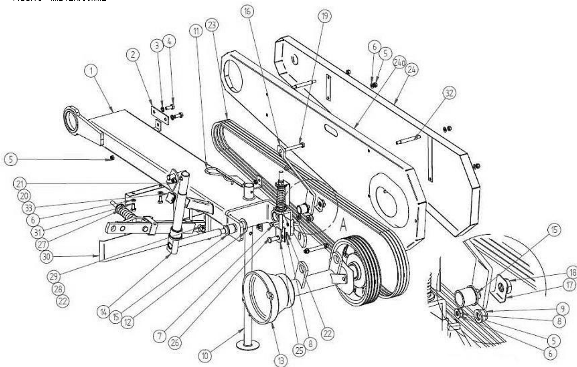
FIGUR 5 – MIDTHERRAMME
