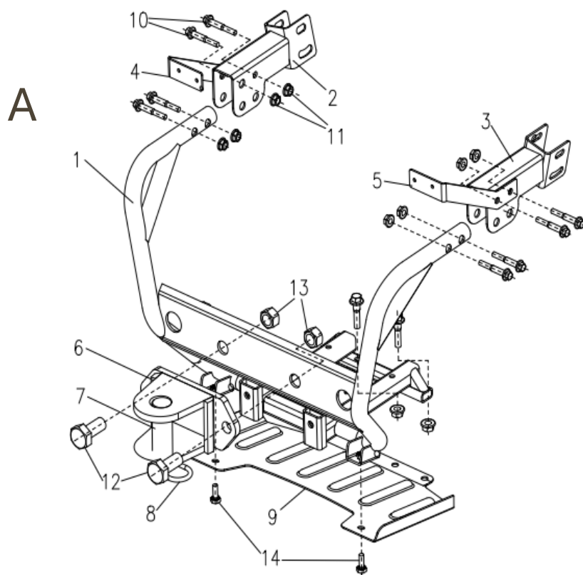
FIGUR 22 – FRONT (A) &amp; KOFANGER (B) / FRONT BUMPER
