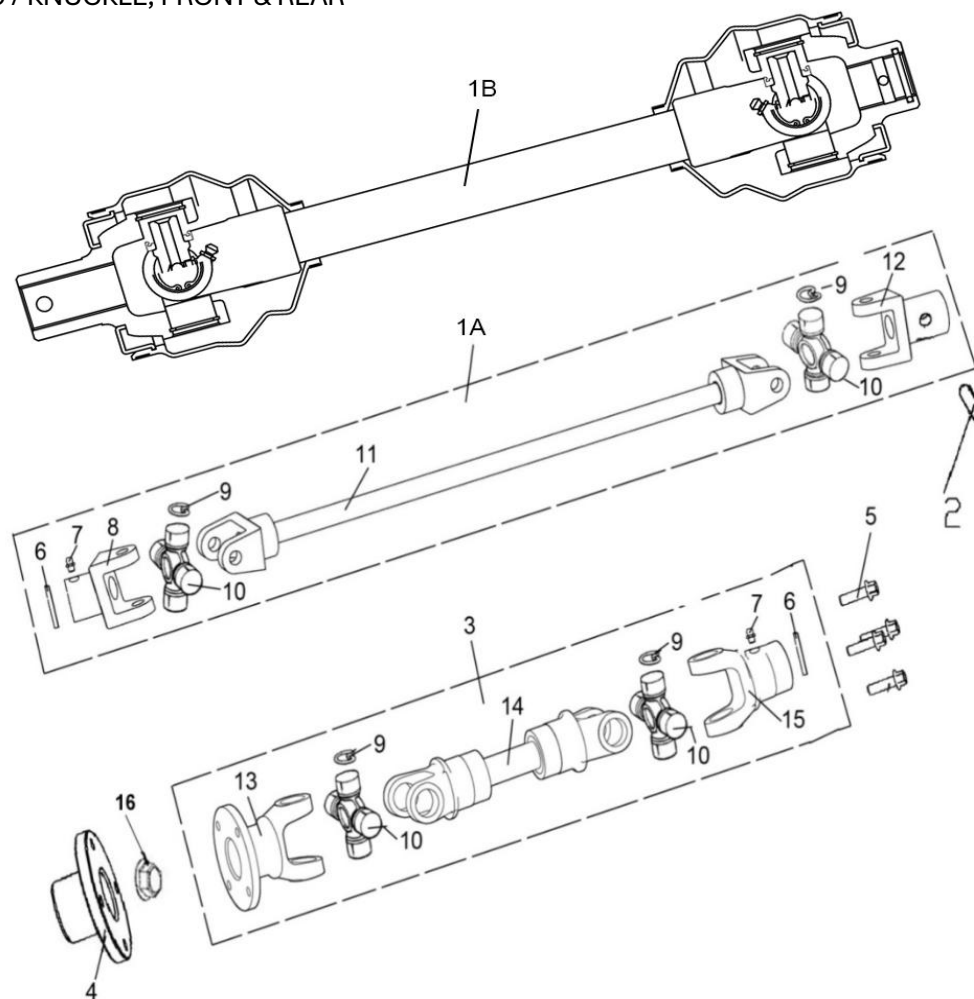
FIGUR 16 – STYRESPINDEL, FRONT &amp; BAG / KNUCKLE, FRONT &amp; REAR
