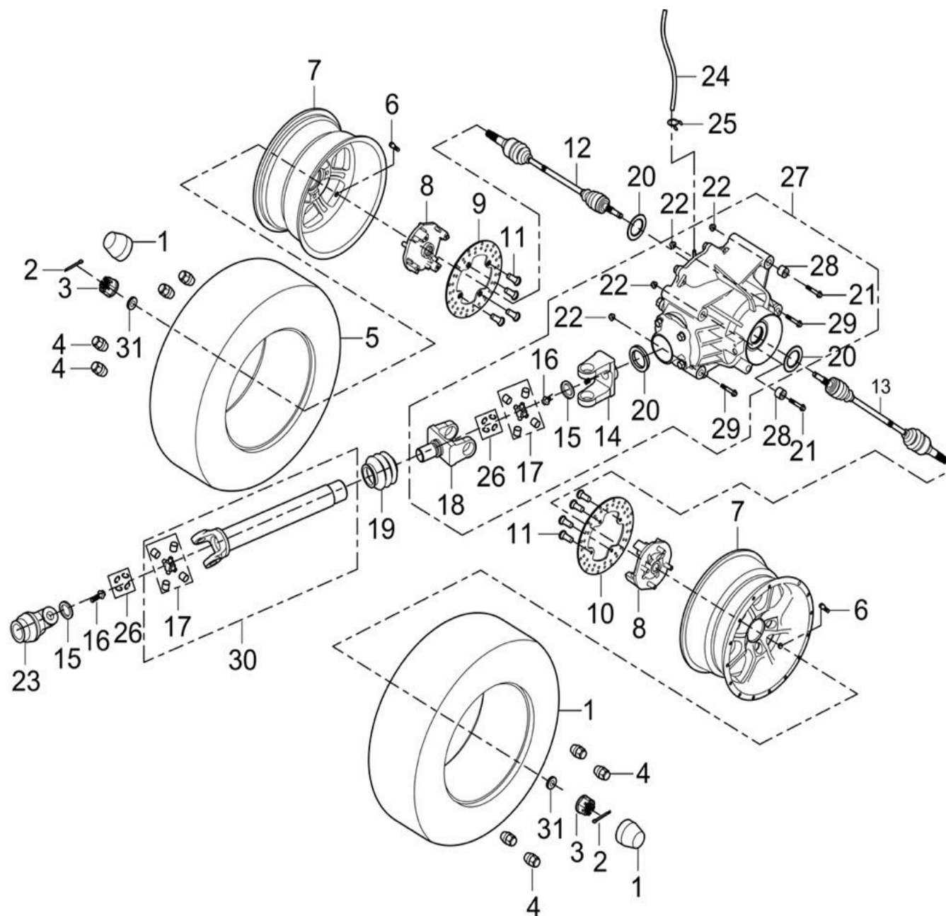
Fig 2: Bagerste differentiale/Rear drive system assembly
