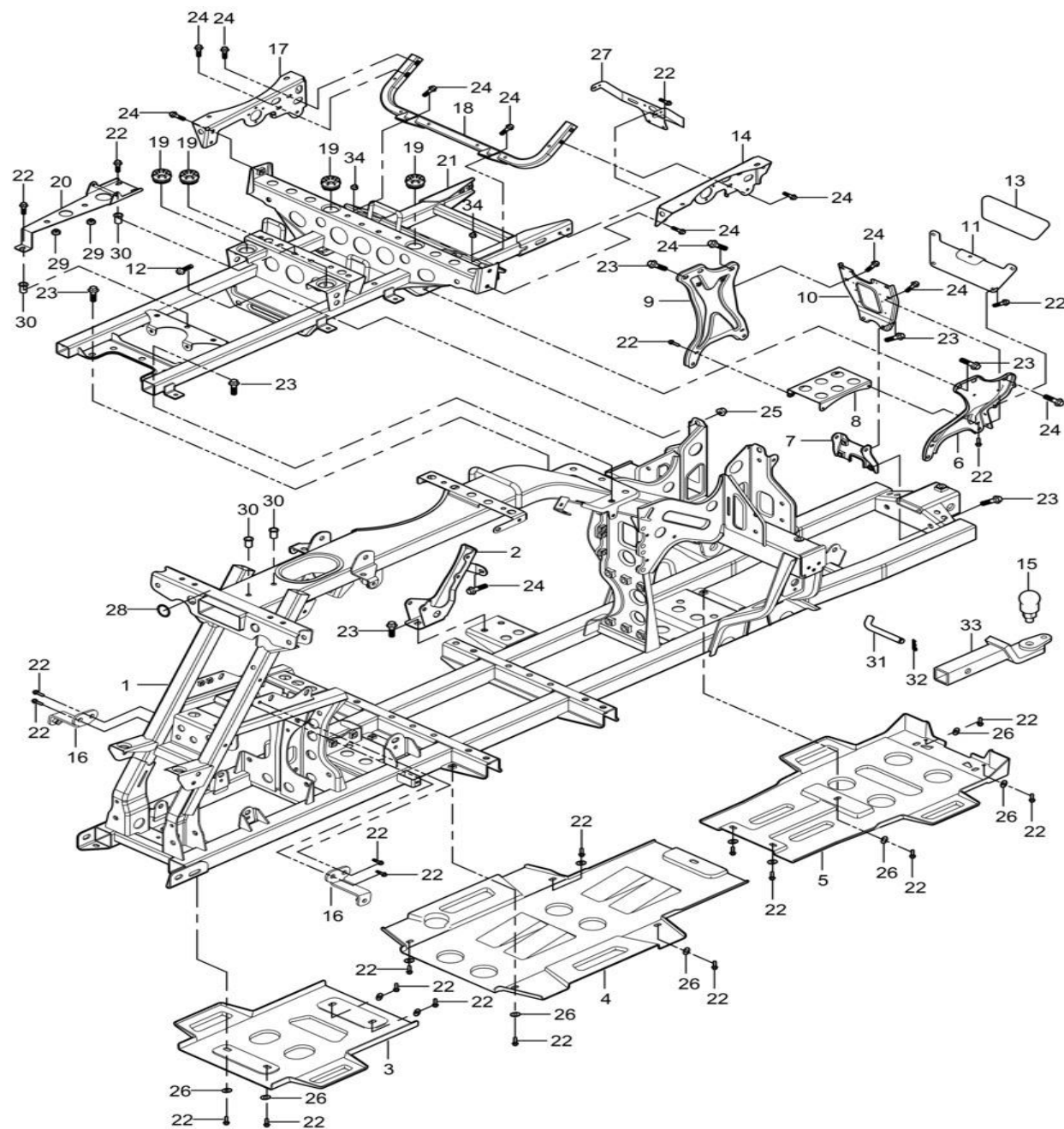
Fig 8: Stel/ramme "lang"/Frame and accessories "long"
