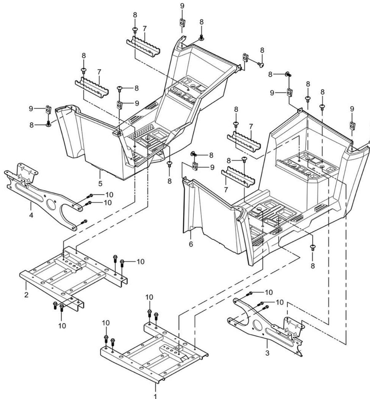
Fig 24: Trinbræt, fodhviler "lang"/Pedal (long)
