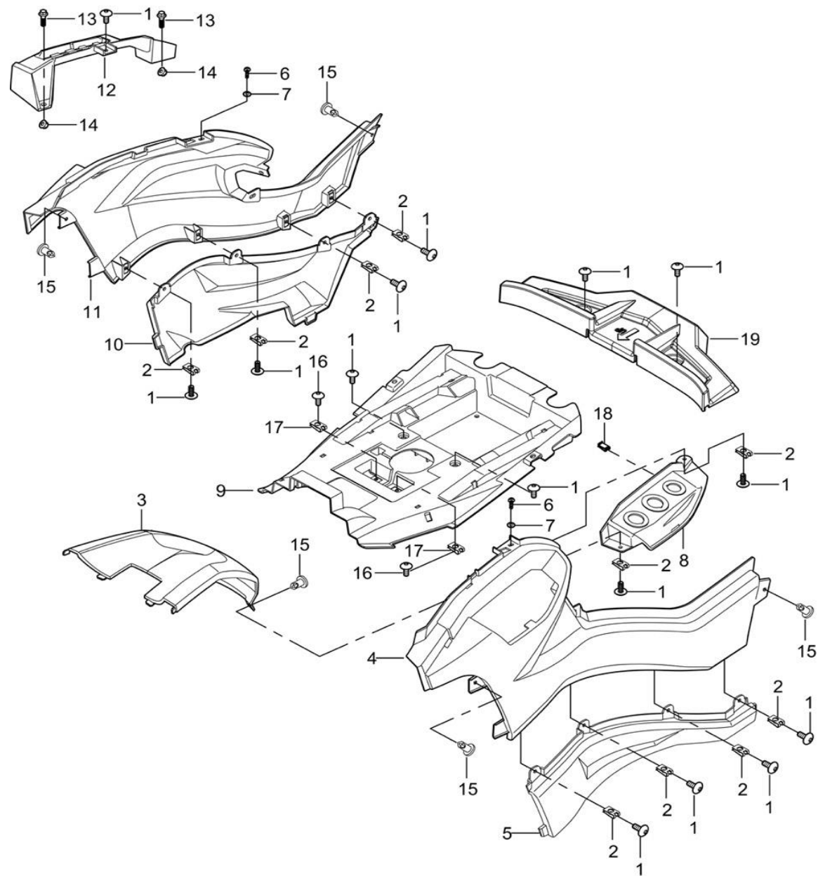
Fig 22: Plastafskærmning, sidedele m.m "kort model"/Side board combination (short)
