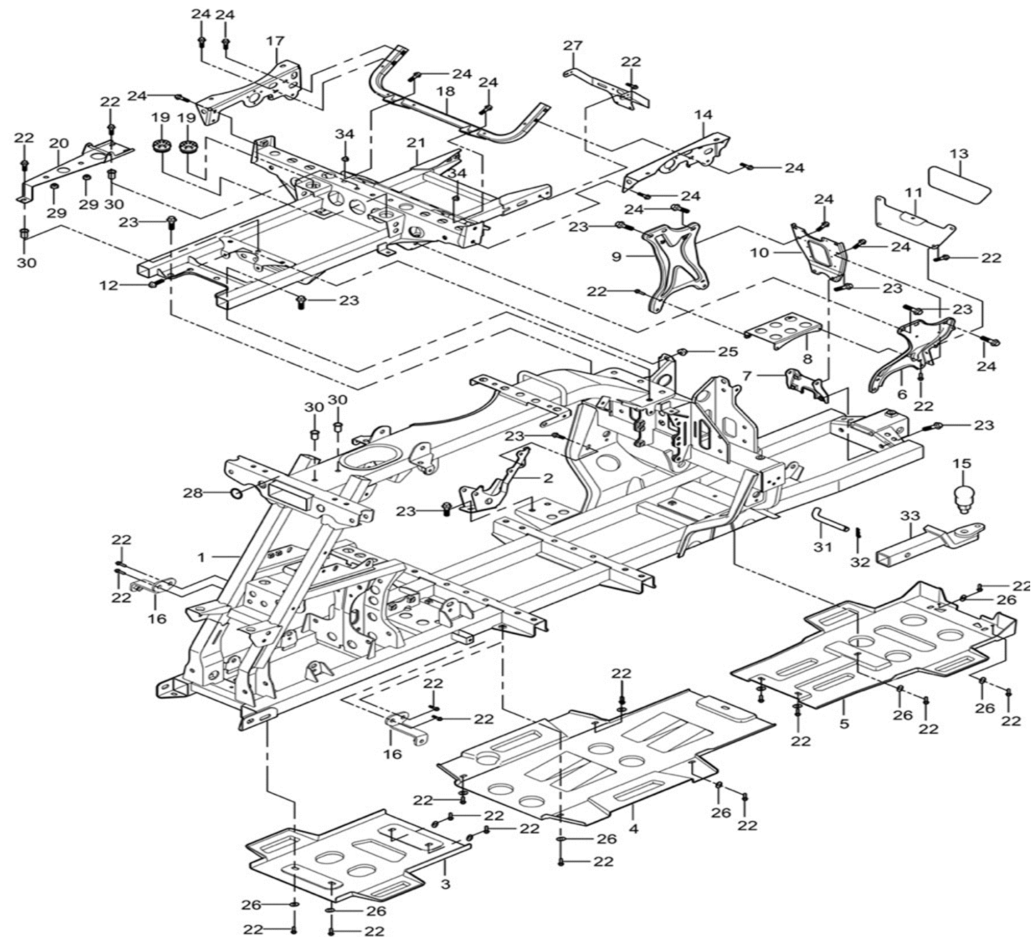
Fig 9: Stel ramme kort/Frame accessories short
