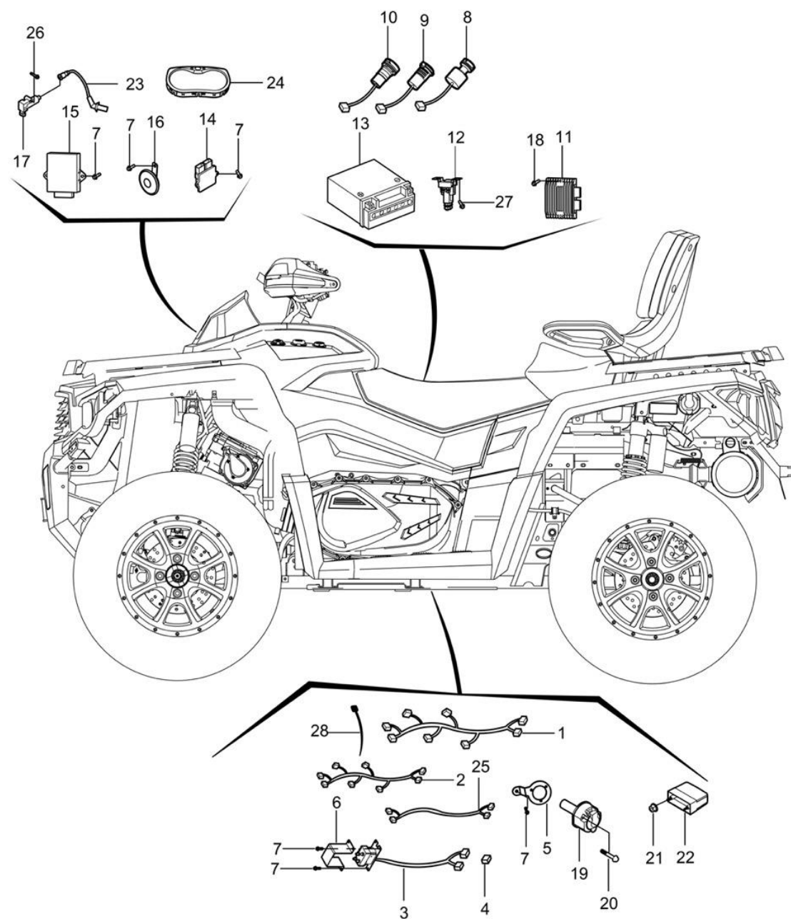
Fig 30: Ledningsnet, sensorer, stik/Electrical parts
