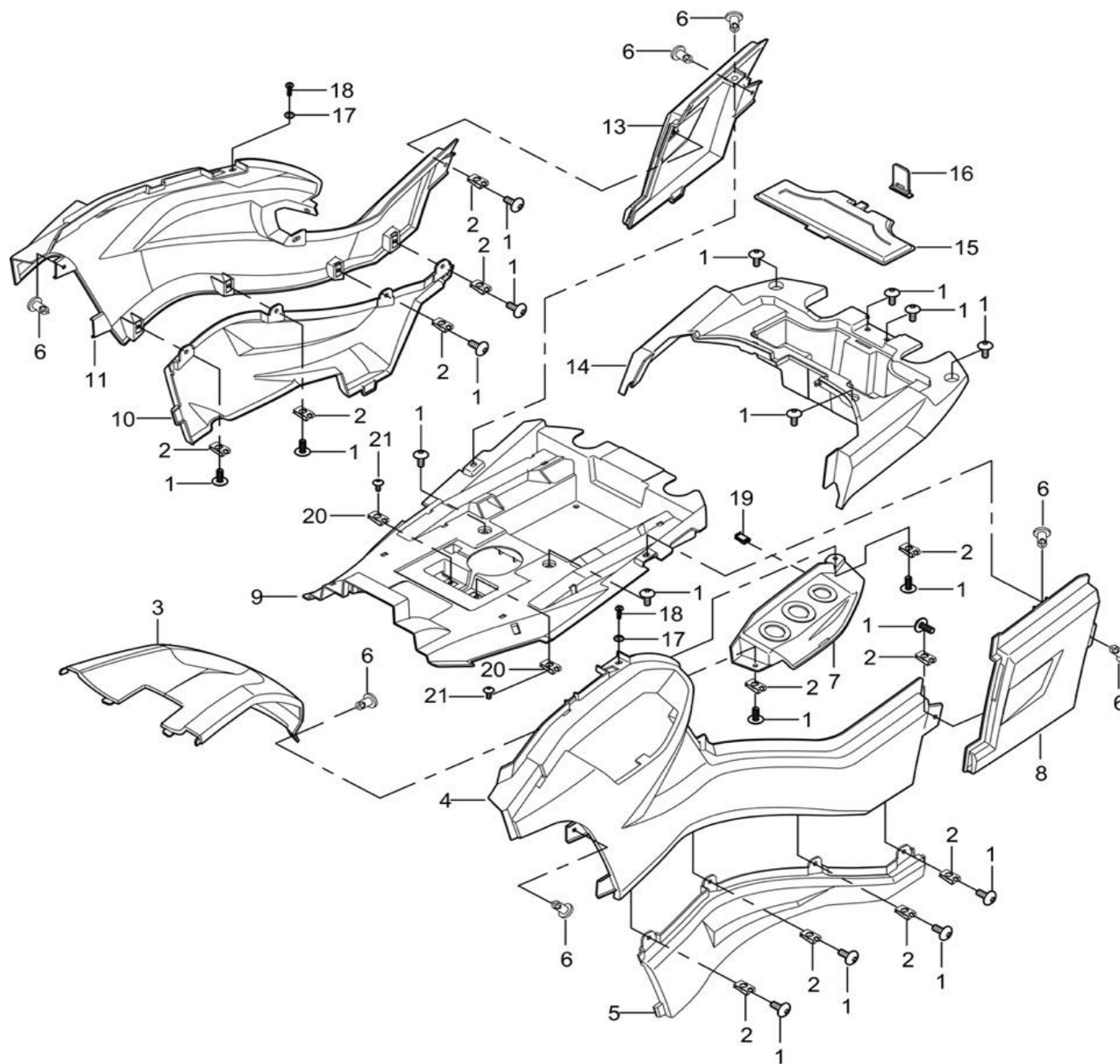
Fig 21: Plastafskærmning, sidedele m.m "lang model"/Side board combination (Long)
