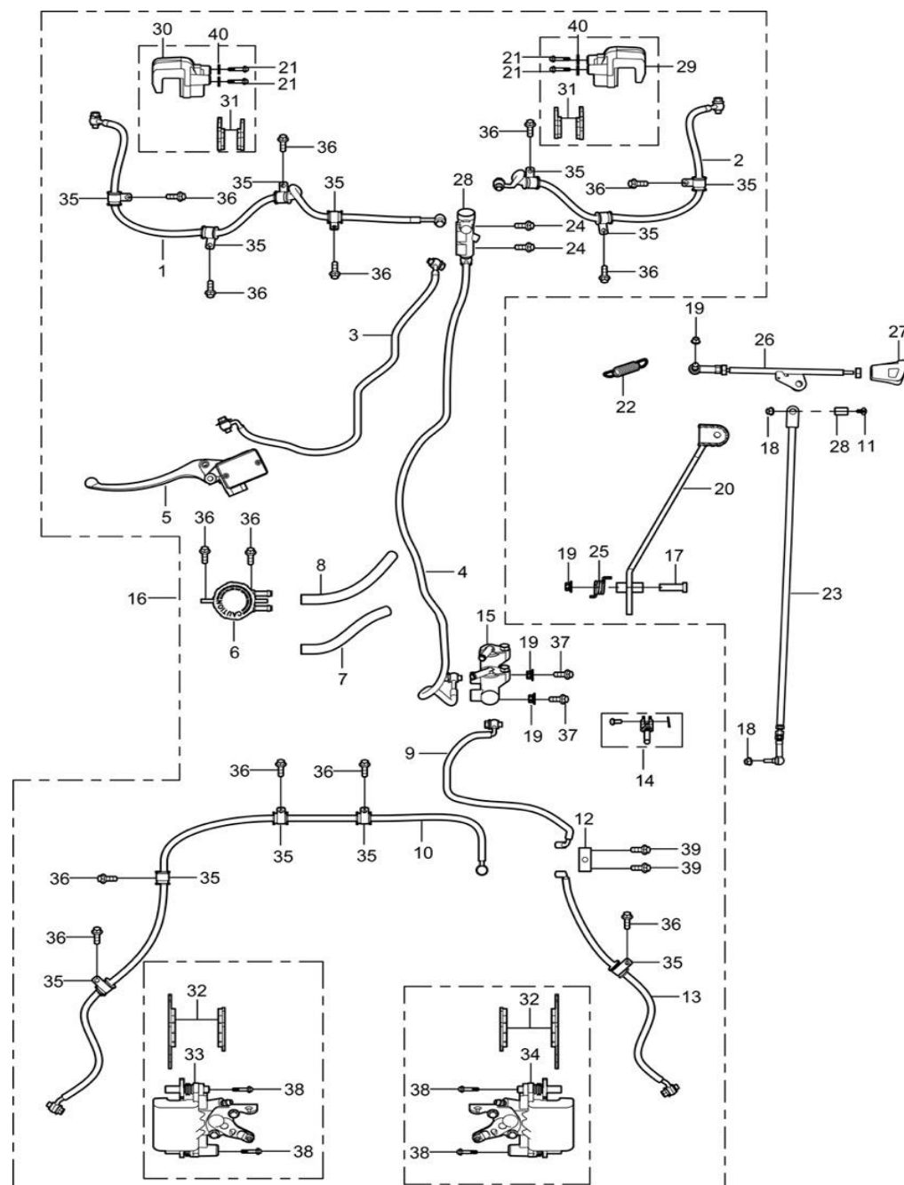
Fig 14: Bremsesystem, gearskifte, kort&lang/Braking system (long&short)
