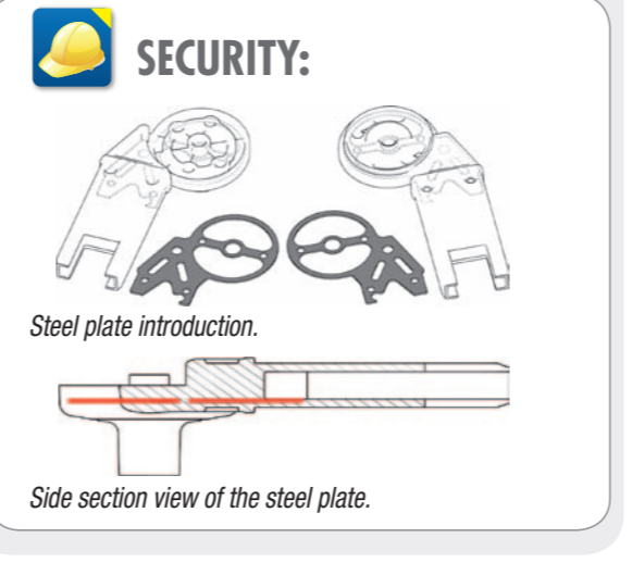
Automatic alum die-casting hinge with an inner steel plate strengthening.
