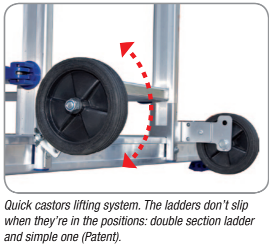
Quick castors lifting system. The ladders don't slip when they're in the positions: double section ladder and simple one (Patent).
