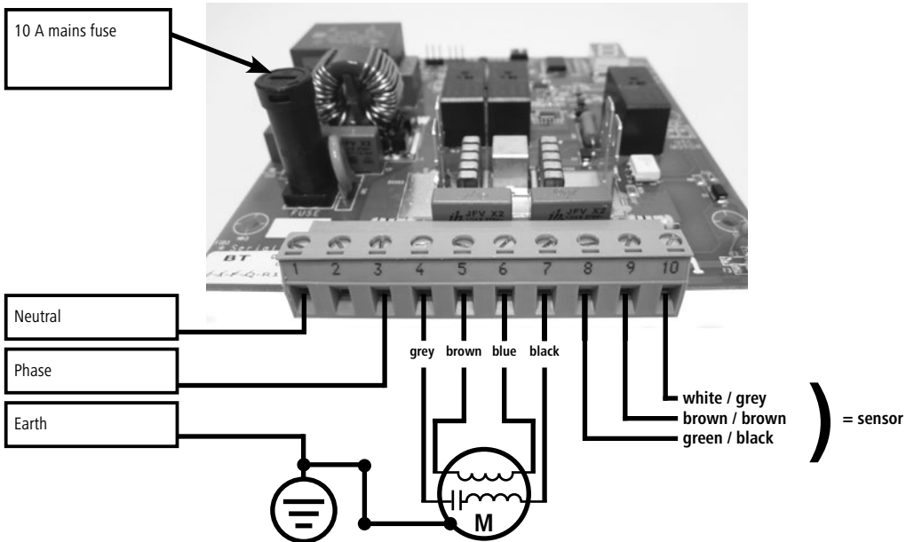
Figure 5: Wiring diagram for HappyCow Swing
