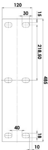
Illustration 2: Monteringshuller
