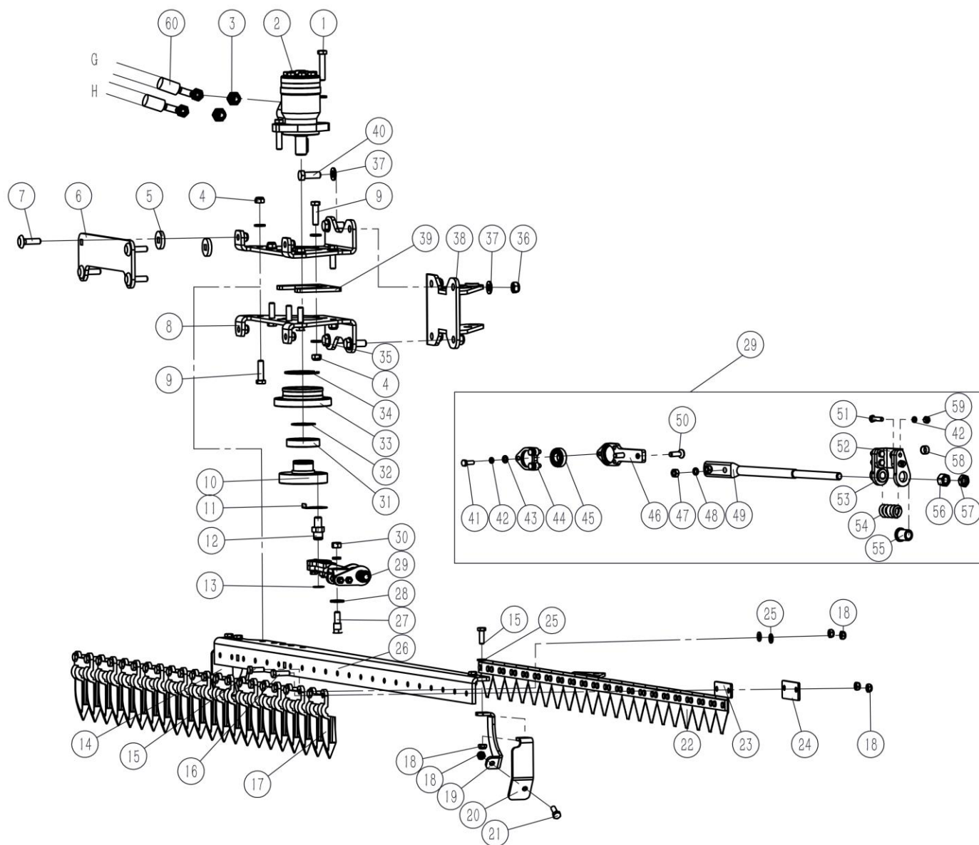
FIG 6 – FINGERKLIPPER T175, 9062935
