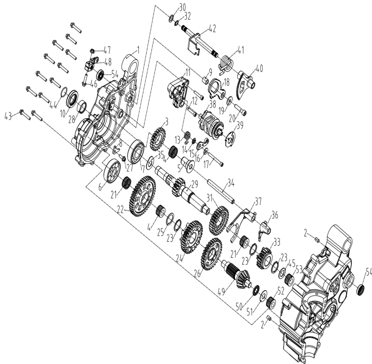
Fig 8: Gearkasse 1 / Gearbox 1
