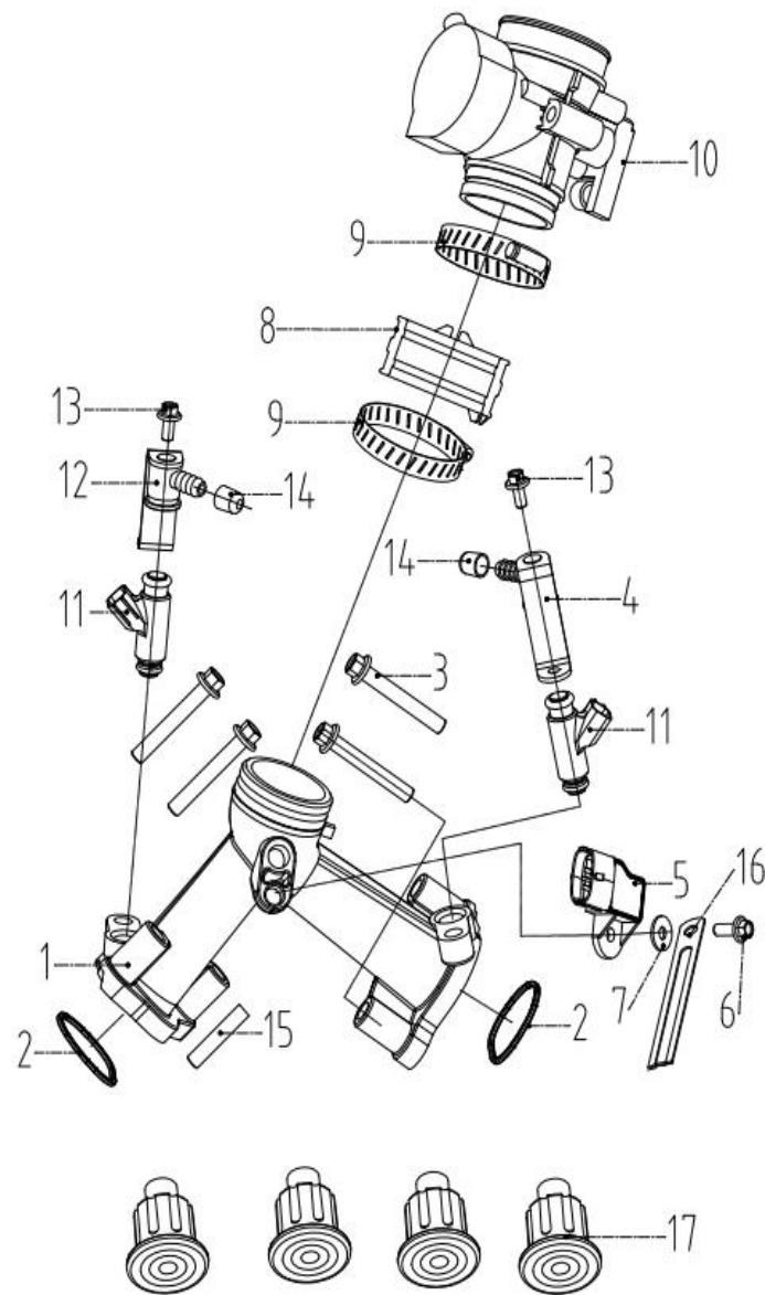
Fig 12: Indsugning, benzindyser, gasspjæld / Air induction system
