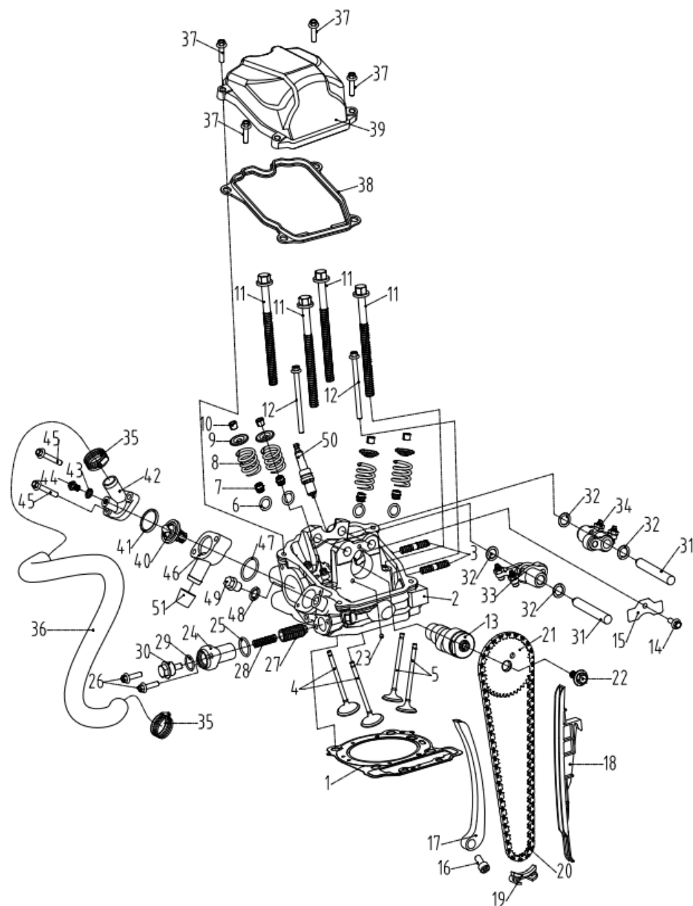
Fig 1: Topstykke Nr 1 / First cylinder head assy
