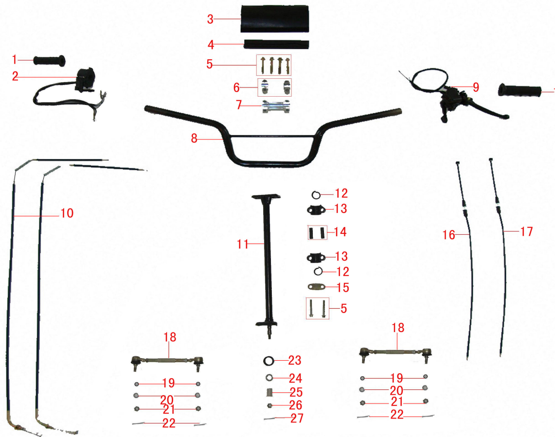
Fig 6: Styringsystem / steering system
