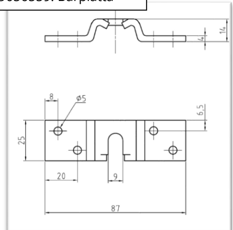
9056559: Bärplatta
