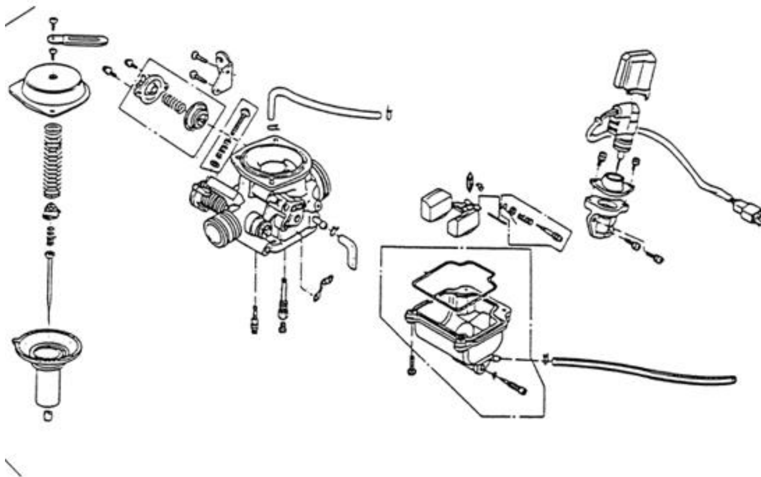
FIG.15 Karburator
