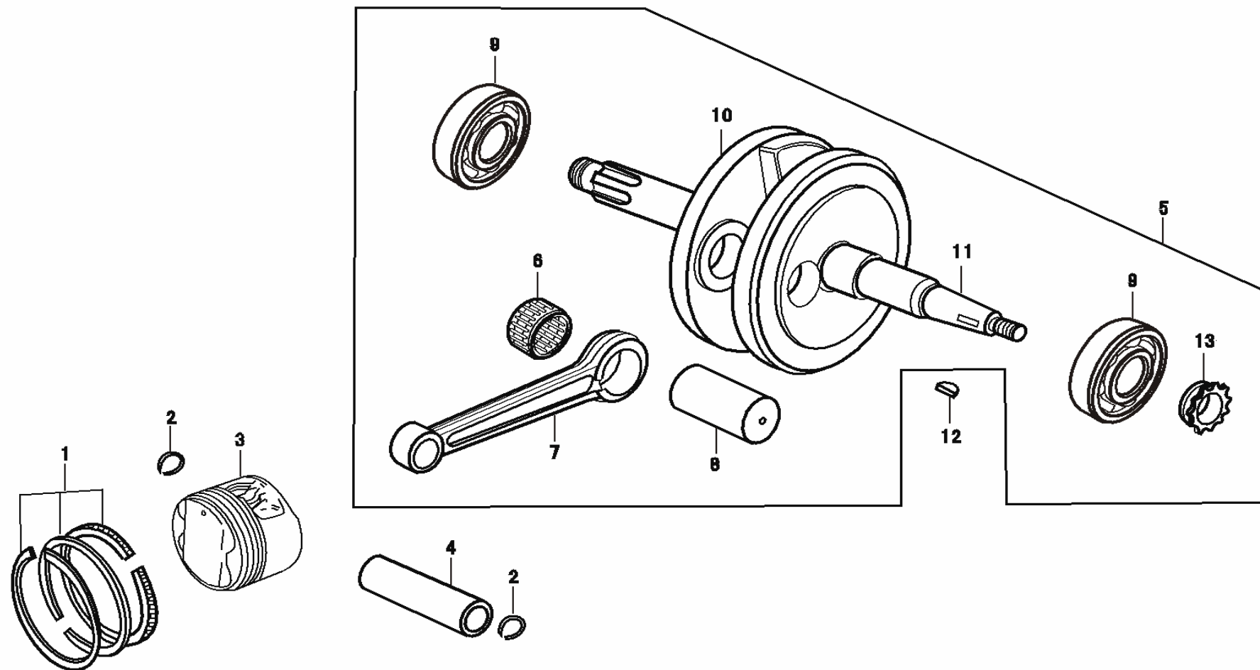
FIG.6 Stempel, krumtap
