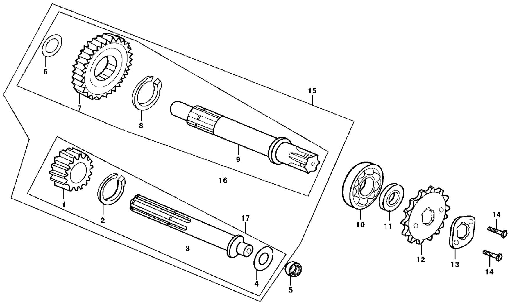
FIG.11 Transmision
