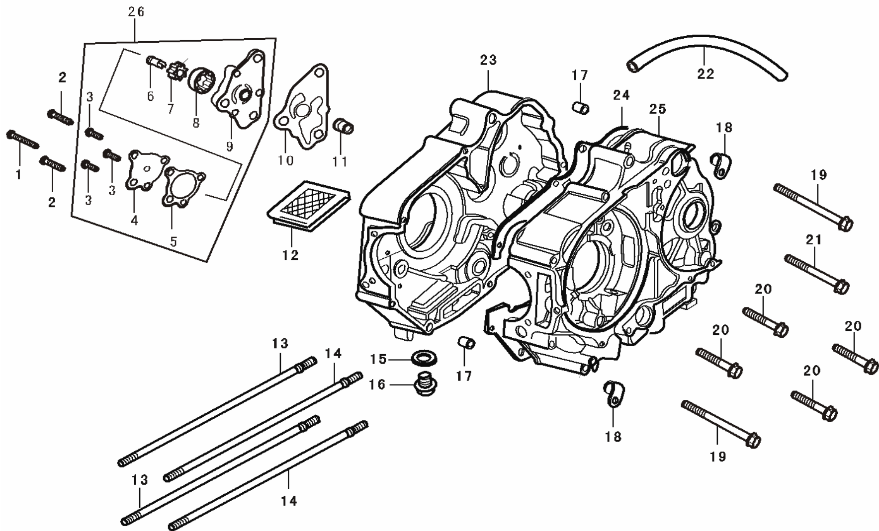
FIG.5 Krumtaphus, oliepumpe
