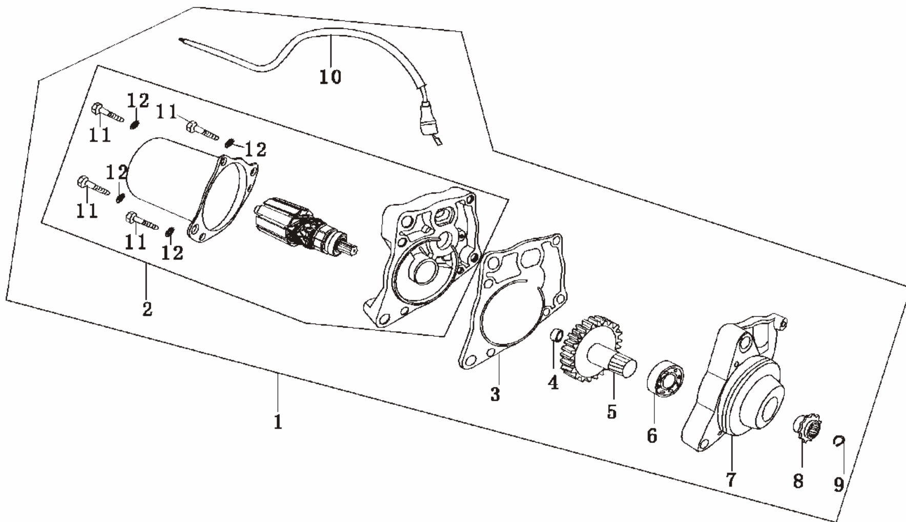
FIG.7 Starter, startdrev
