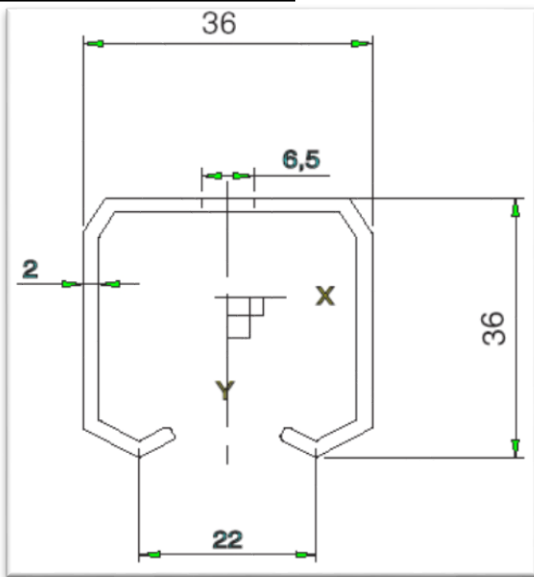
9014214: Portskena
