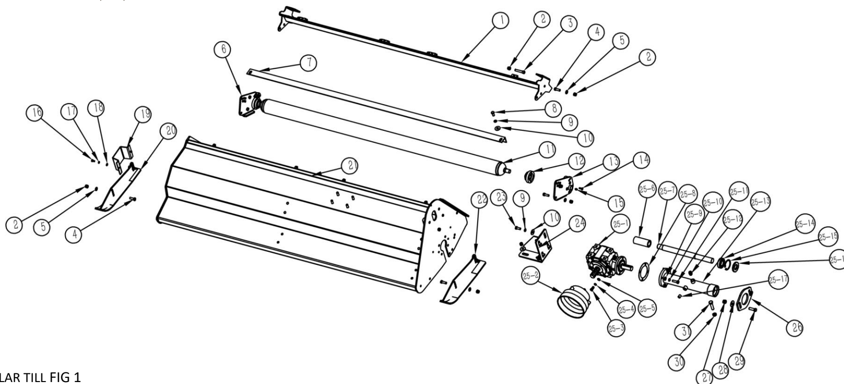
FIG 1 – AHEAD NBM 105, 155, 175
