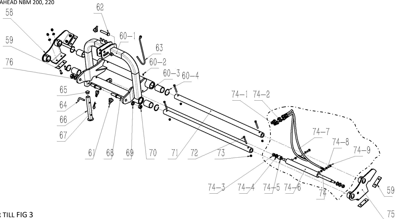
FIG 3 – AHEAD NBM 200, 220
