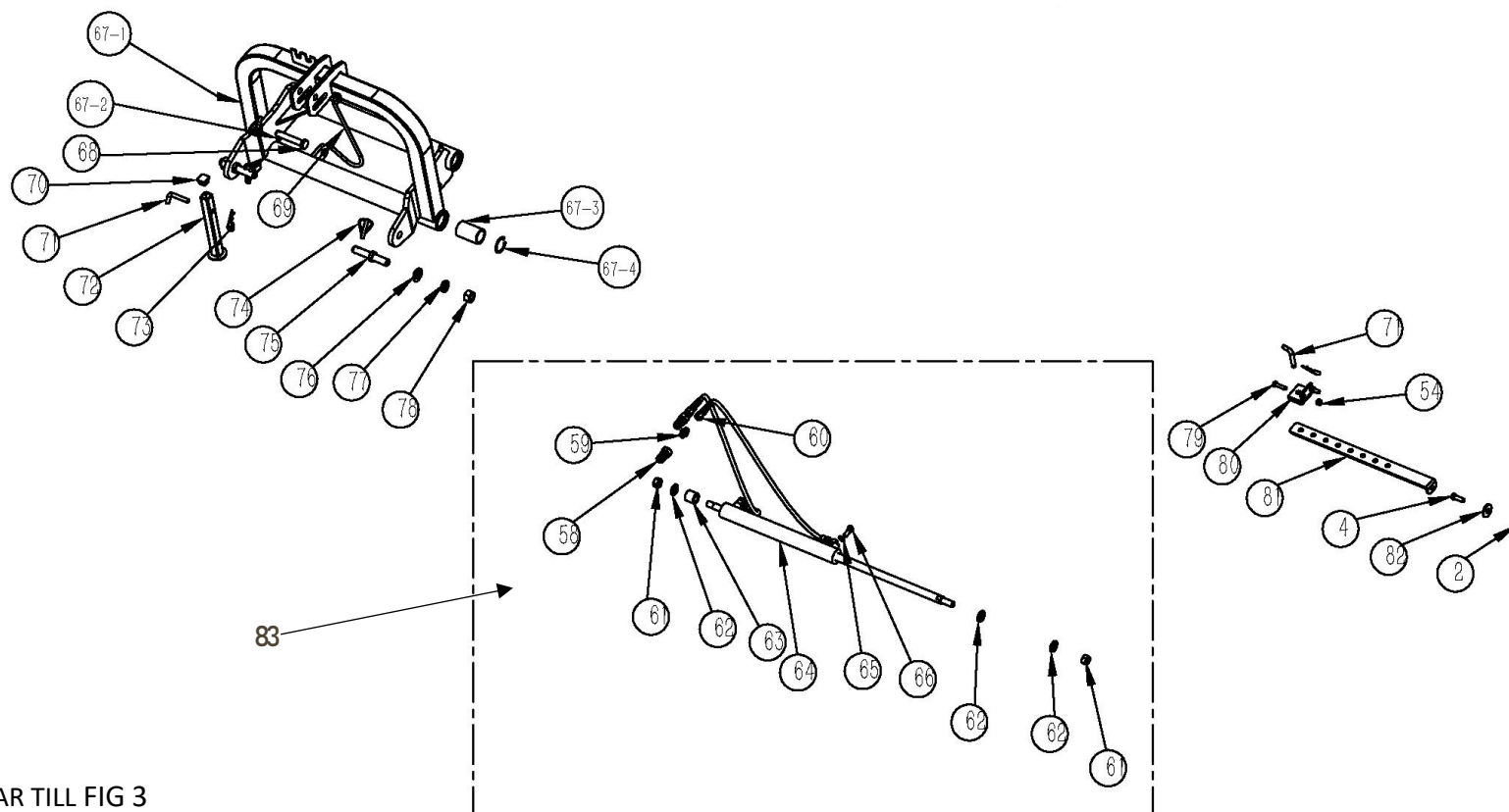
FIG 3 – AHEAD NBM 105, 155, 175
