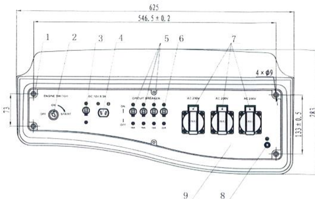
FIGUR 5 – KONTROL PANEL / CONTROL PANEL
