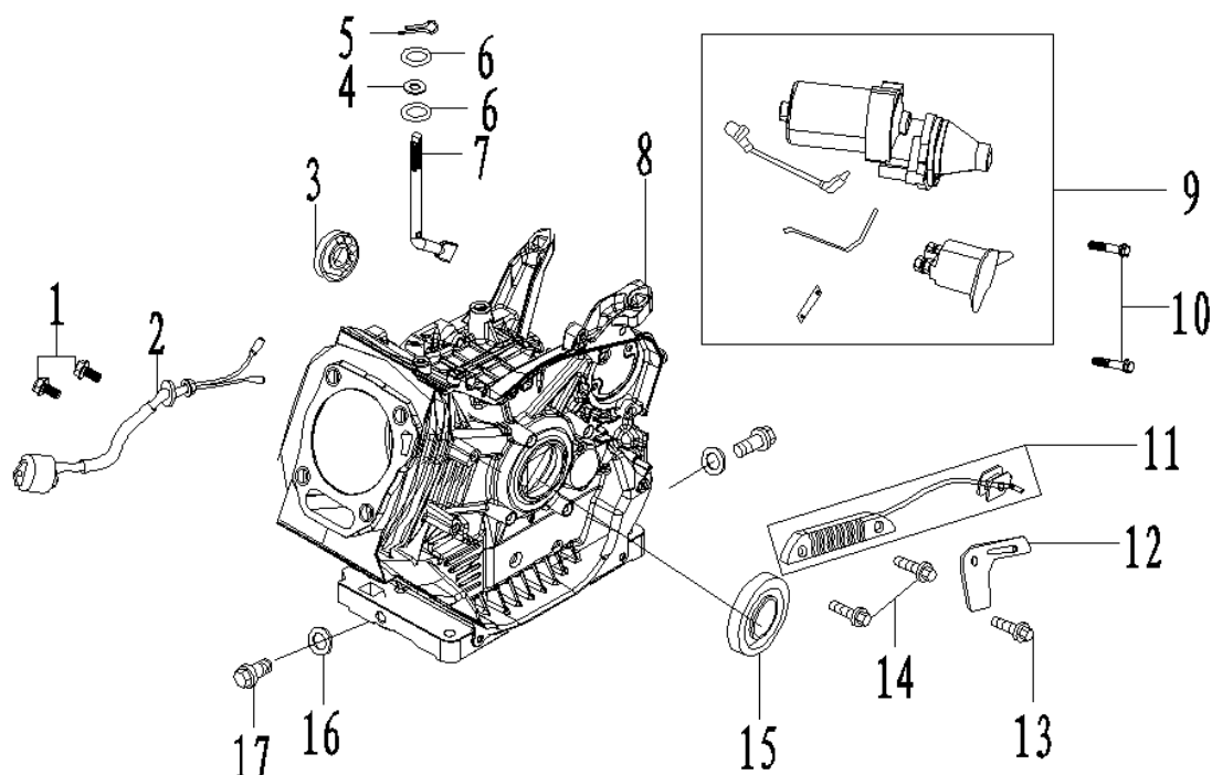
MOTOR FIGUR 2 – KRUMTAPHUS / CRANKCASE
