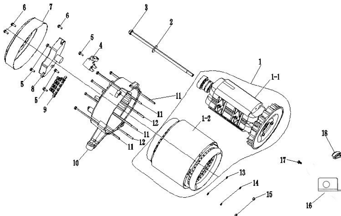
FIGUR 3 – MOTOR / ENGINE
