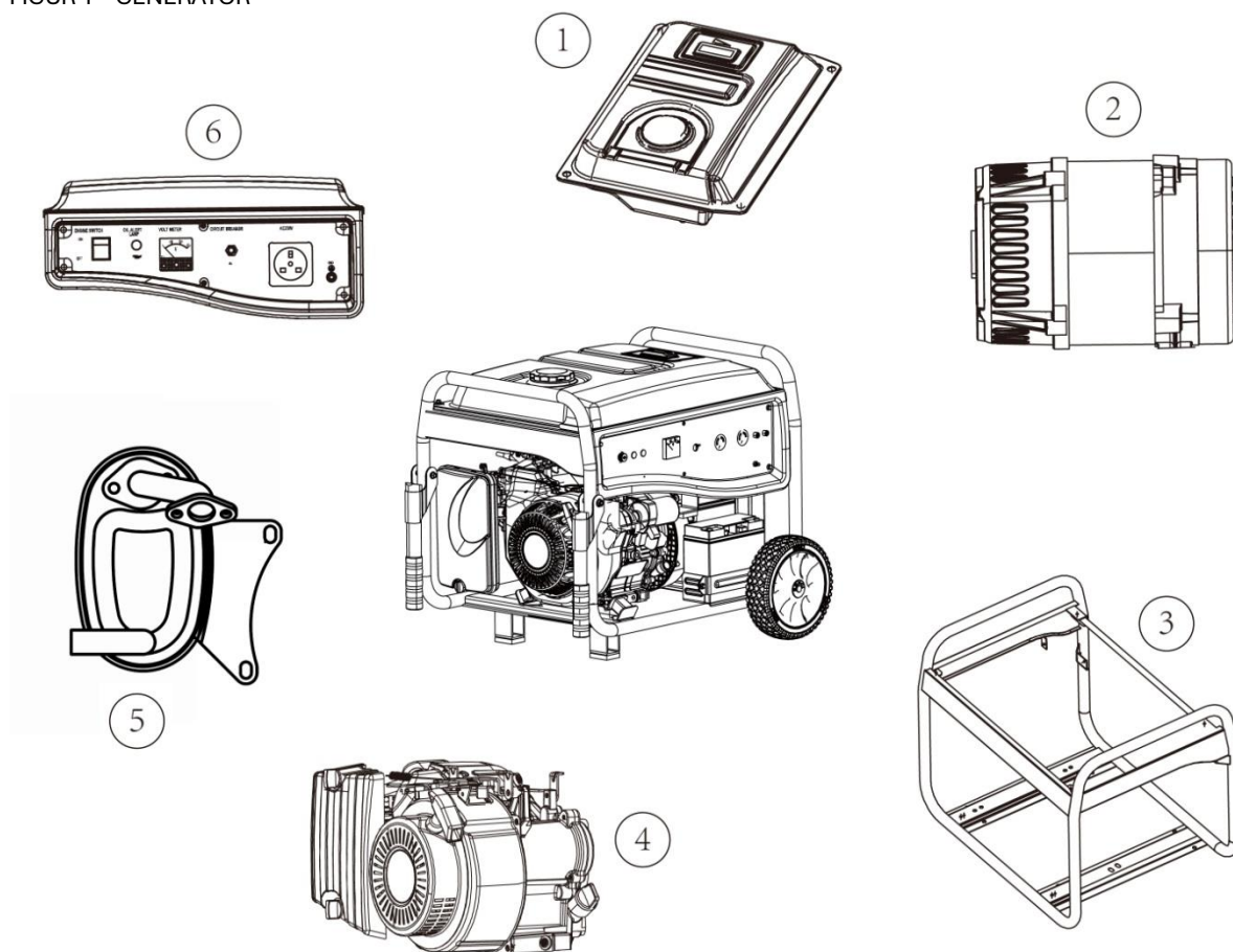
FIGUR 1 – GENERATOR
