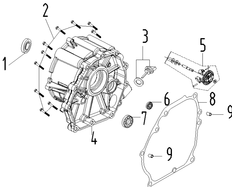
MOTOR FIGUR 3 – KRUMTAPDÆKSEL / CRANKCASE COVER
