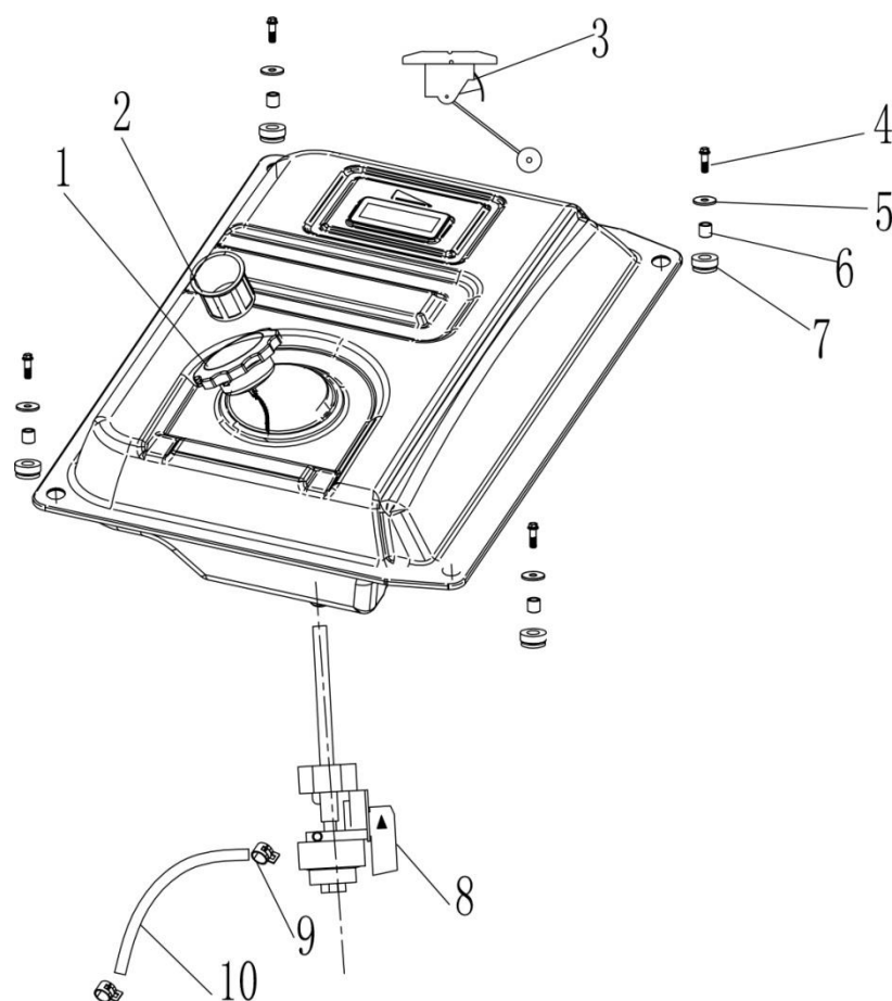
FIGUR 2 - BENZINTANK / FUEL TANK
