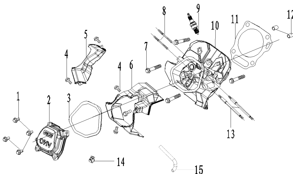
MOTOR FIGUR 1 – CYLINDER / CYLINDER HEAD
